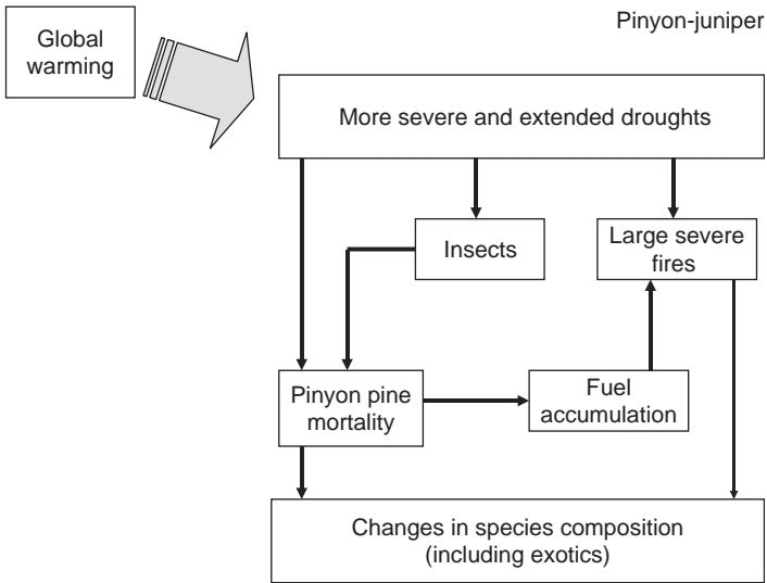
Figure 15.3. Stress complex in pinyon-juniper woodlands of the American Southwest. The effects of disturbance regimes (insects and fire) are exacerbated by global warming. Stand-replacing fires and drought-induced mortality both contribute to species changes and exotic invasions.
