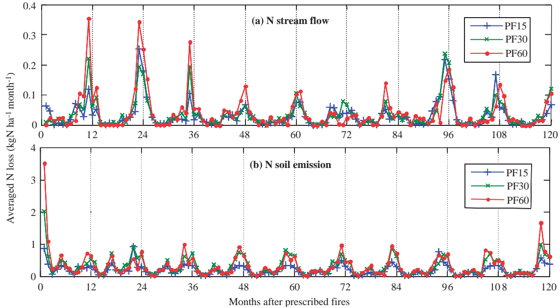
Figure 19.11. N in stream flow (a) and soil trace gas emissions (b) after prescribed fires (PF) under a deposition scenario of 25 kg N ha -1 yr -1 and considering three different PF intervals: 15 years (blue line), 30 years (green line), and 60 years (red line).
