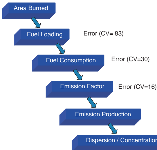
Figure 3.1. Information required for estimating emission production. The largest errors are associated with fuel loading and fuel consumption inputs (Peterson, 1987) unless the area burned is total acres within the perimeter of the fire. (CV = coefficients of variation.)
