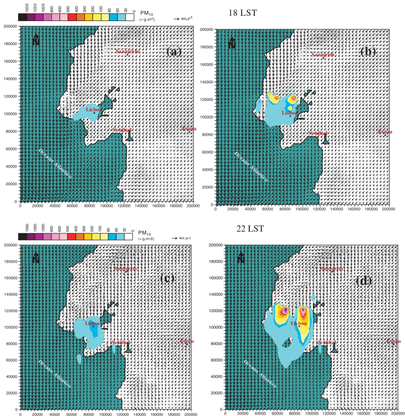
Figure 9.8. Hourly averaged surface PM_{10} concentration ( \mu\text{g}\cdot\text{m}^{-3} ) and wind values at 18.00 (a, b) and 22.00 (c, d) LST, both excluding forest fire emissions (a, c) and including forest fire emissions (b, d) in Lisbon.
